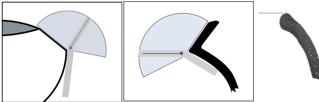
Figure 24. Left: Goniometer measurement of an inverted rim bowl with clear inflection point; middle: goniometer measurement of an everted rim jar; right: an example of an unmeasurable rim angle, with no inflection point.
