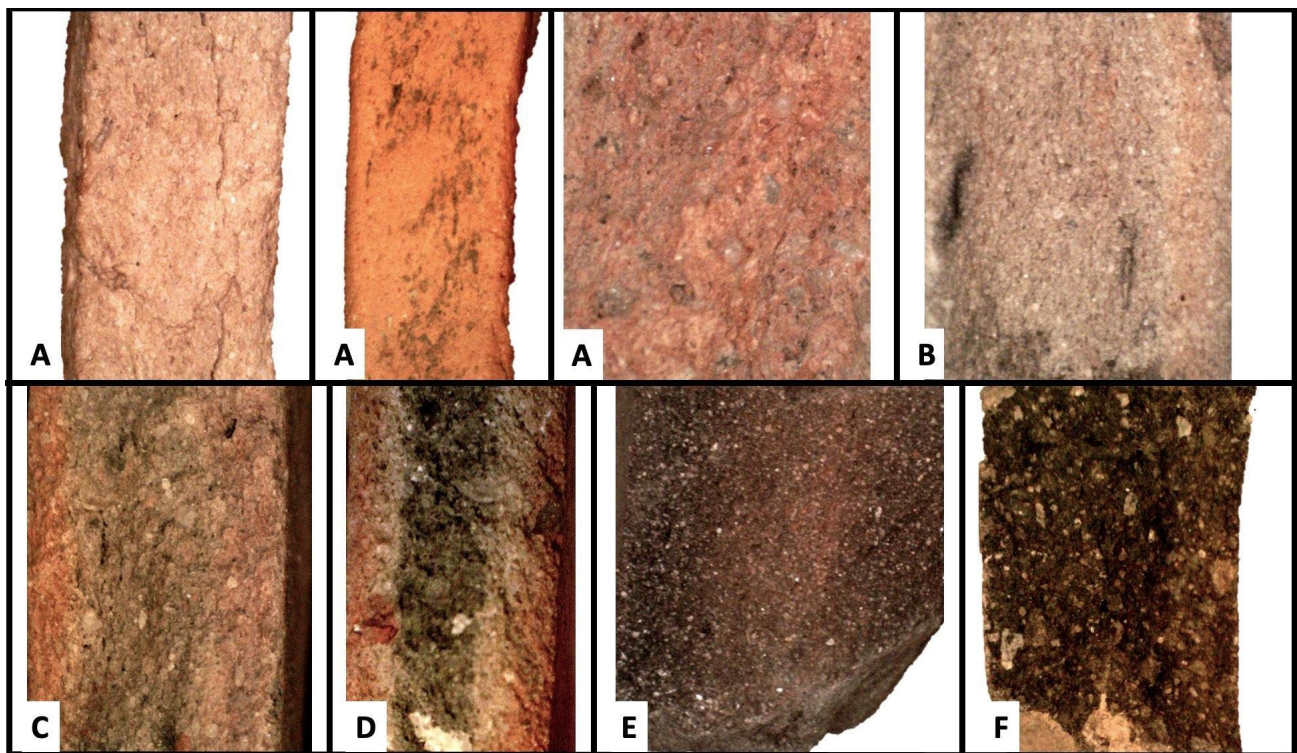
Figure 31. Examples of reduction patterns in sherd cross-sections. A: Oxidized, AKA “Not Reduced;” B: light bands of uneven reduction/oxidation; C: oxidized exteriors with diffuse reduced core; D: oxidized exteriors with sharp reduced core; E: reduced exteriors with oxidized core; F: fully reduced paste.
